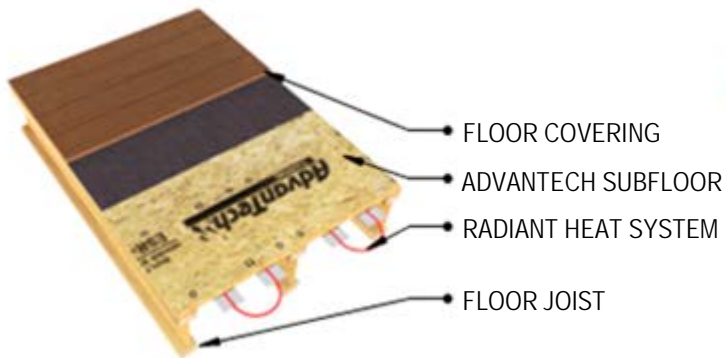
Electric Roll Heating System Below Subfloor
