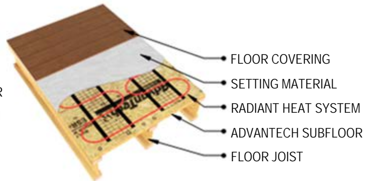
Radiant Heating System Above Subfloor
